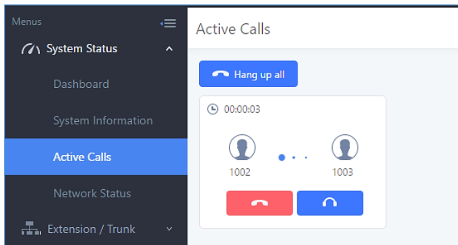
Figure 212: Status→PBX Status→Active Calls – Call Established
