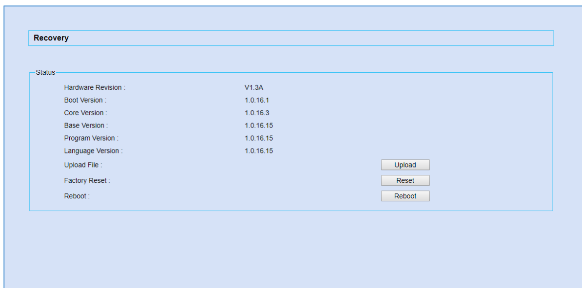
Figure 316: Recovery Mode
