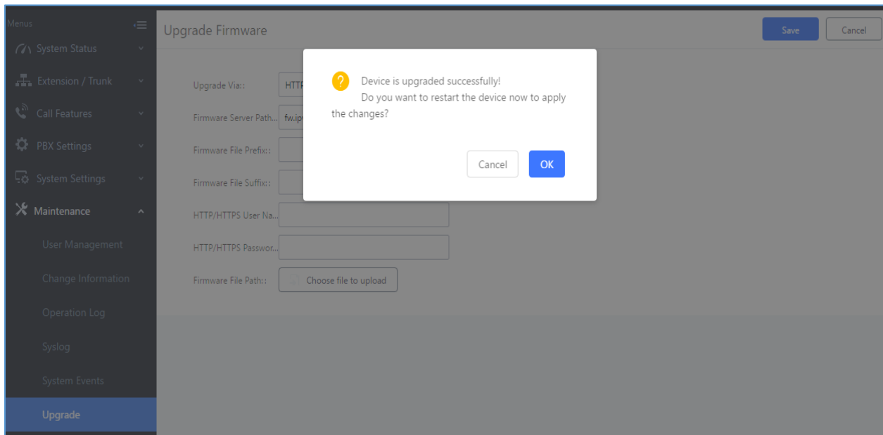
Figure 306: Reboot UCM6510
