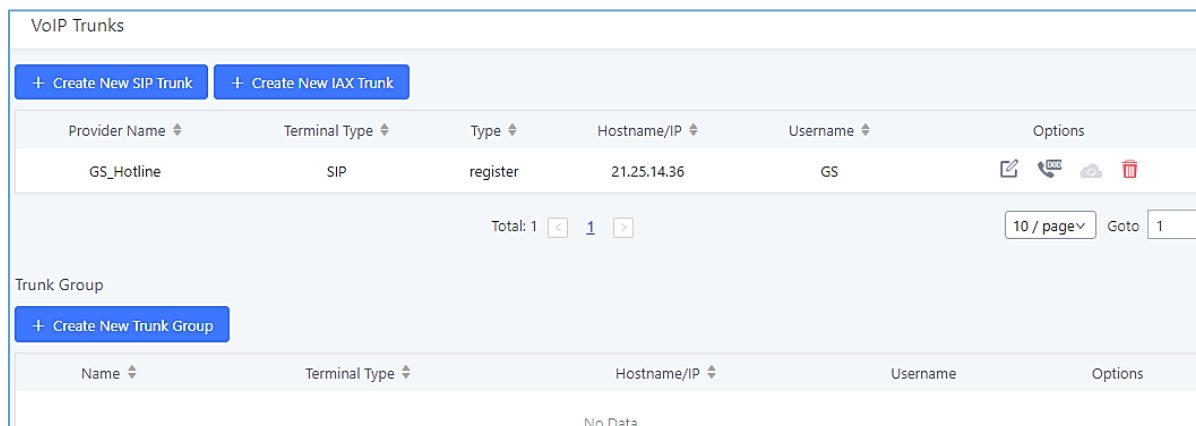
Figure 106: Trunk Group
