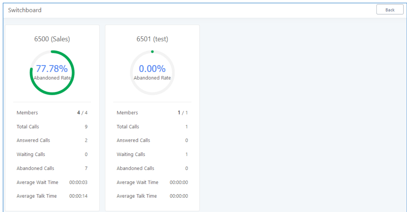
Figure 177 : Switchboard summary
