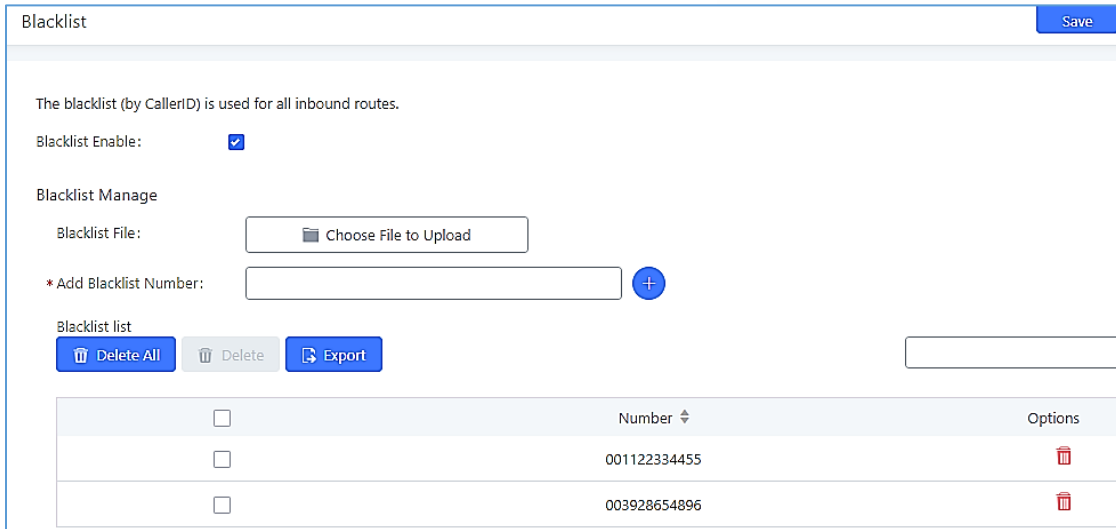
Figure 133: Blacklist Configuration Parameters
