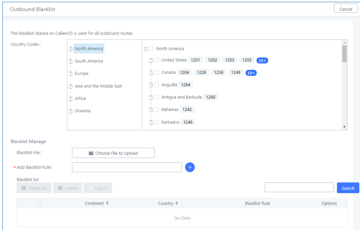
Figure 115: Country Codes
