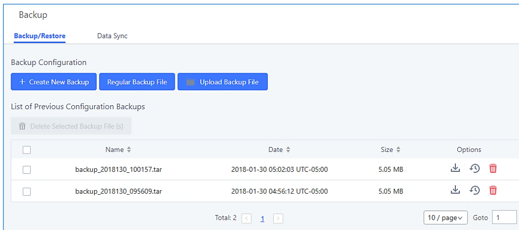
Figure 308: Backup / Restore
