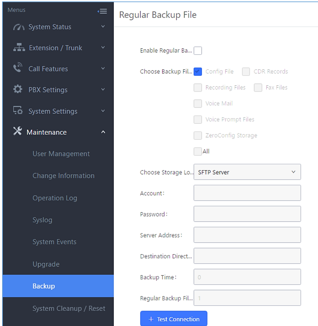
Figure 309: Local Backup
