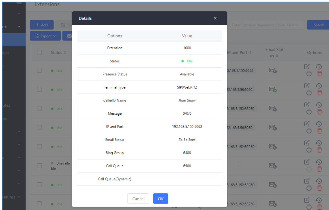
Figure 86 : Extension Details
