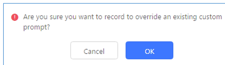
Figure 187: Information Prompt
