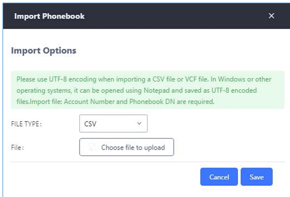
Figure 35: Import Phonebook
