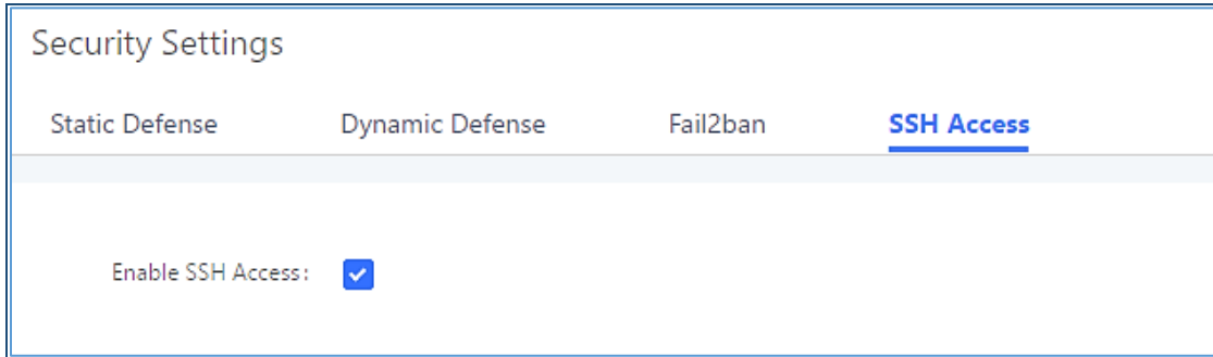
Figure 29: SSH Access
