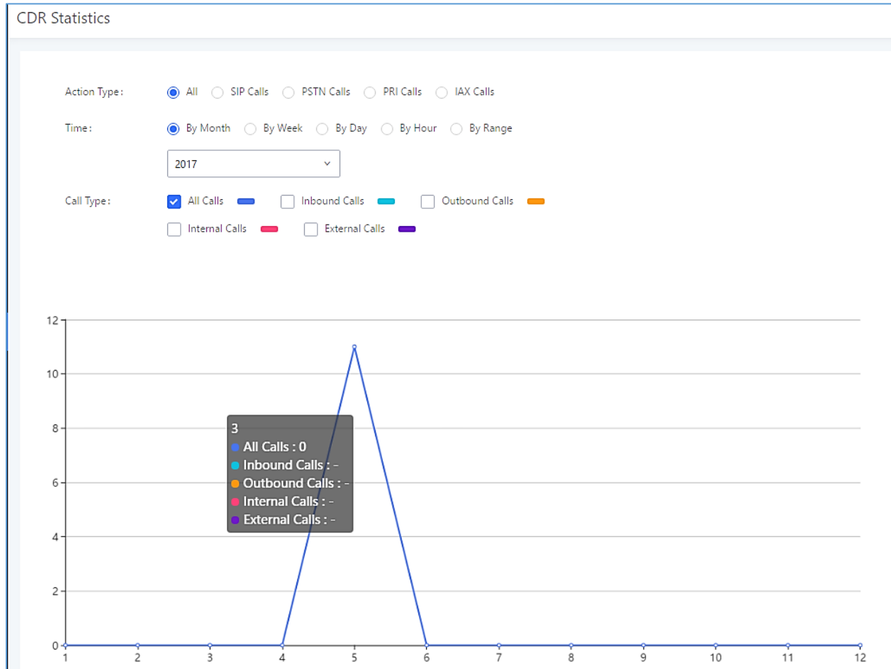
Figure 286: CDR Statistics
