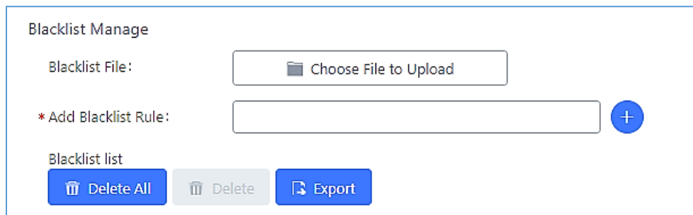
Figure 116: Blacklist Import/Export
