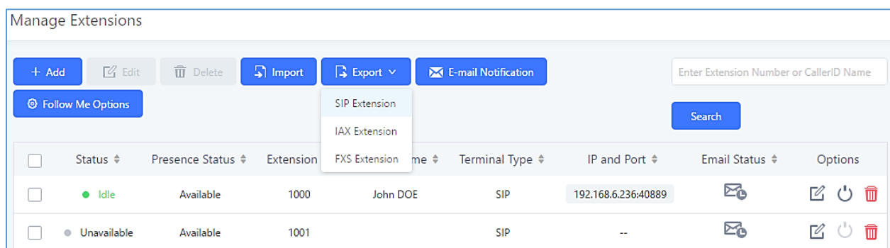
Figure 82: Export Extensions
