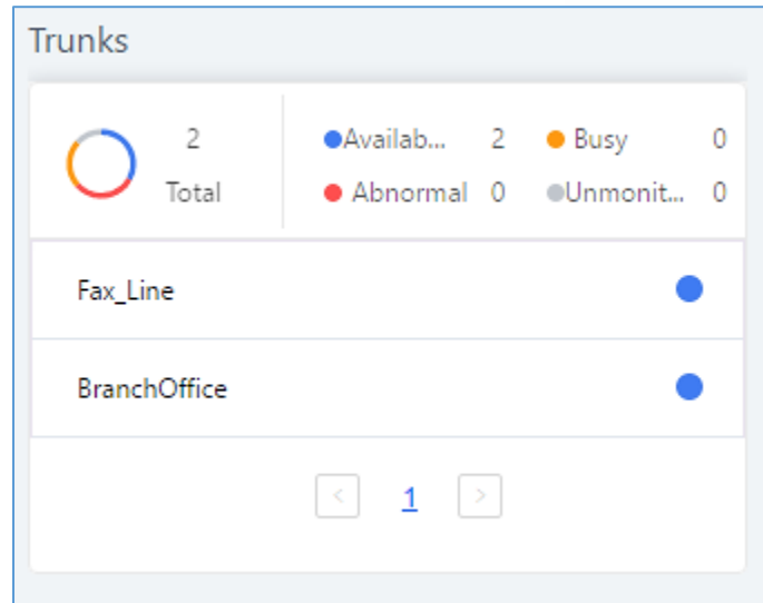
Figure 265: Trunk Status
