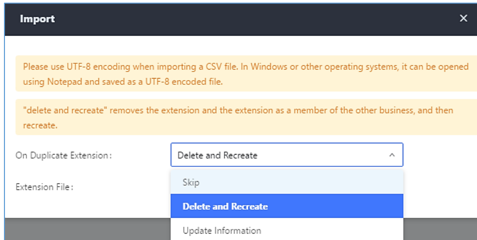
Figure 83: Export Extensions
